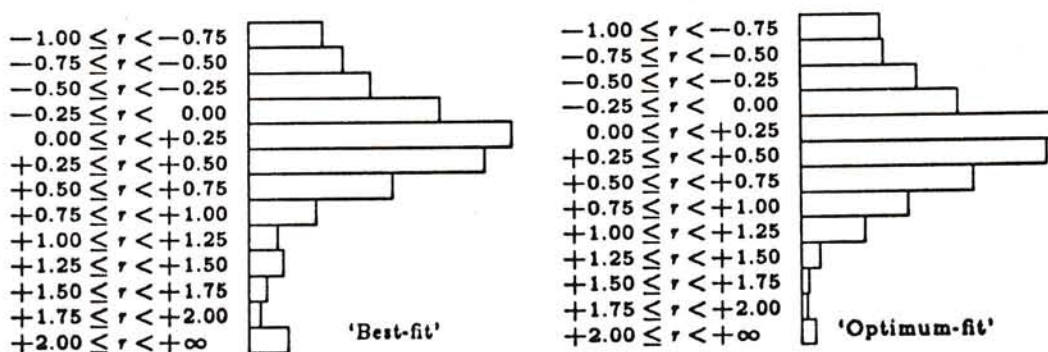
Figure 20. The distribution of interword spaces found by the best line-at-a-time method, compared to the distribution found by the best paragraph-at-a-time method, when difficult mathematical copy is typeset without human intervention.
